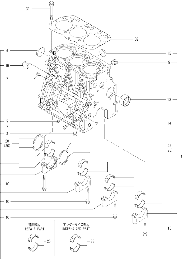
0CW10-M31500 3TNV84T-BGGE Fig.1. CYLINDER BLOCK
