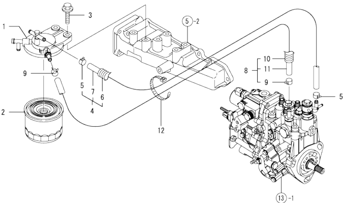
Fig.16. FUEL LINE
